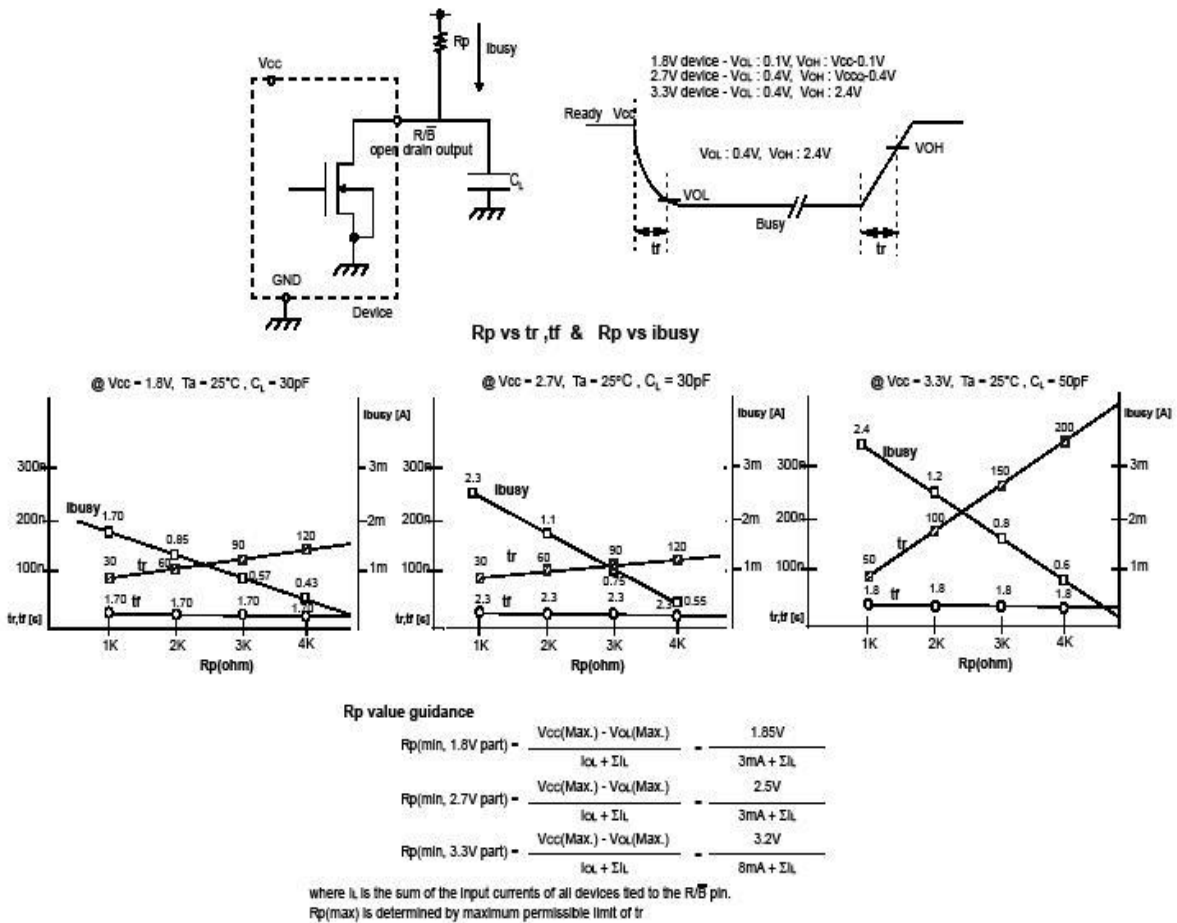
Figure 32 : Ready/Busy Pin electrical application
