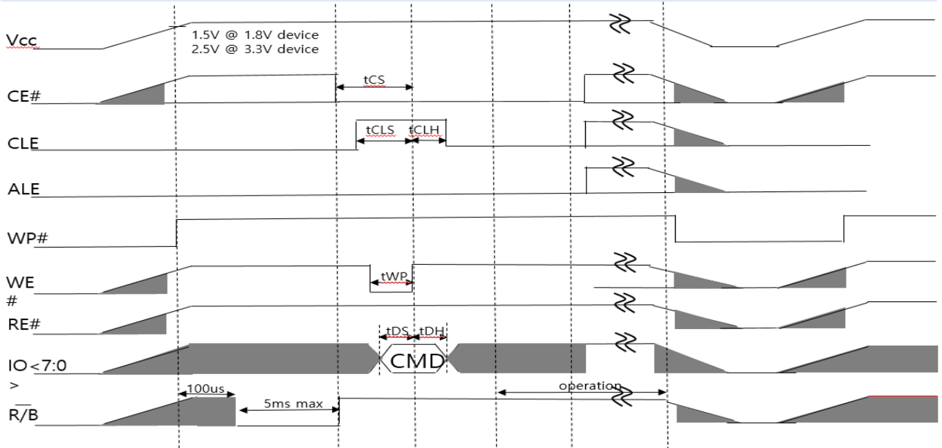
Figure 31 : Power up time sequence
